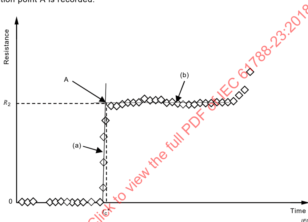
Figure A.1 – Determination of the value of R_2 from a resistance versus time plot
