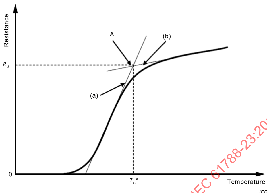
Figure 1 – Relationship between temperature and resistance near the superconducting transition
