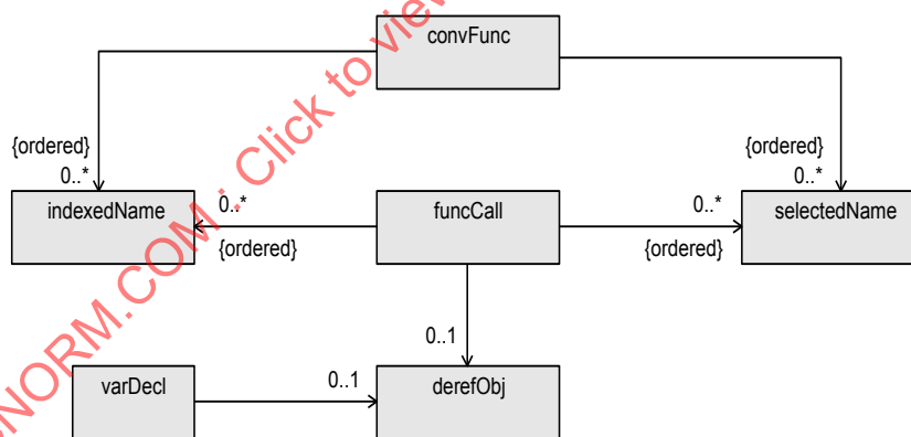
Figure 7—Composite class diagram
