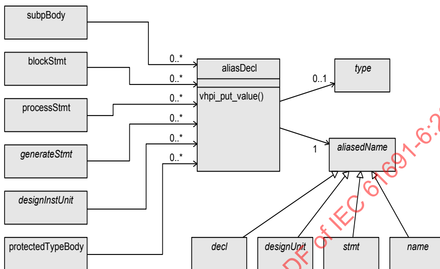
Figure 6—AliasDecl class diagram
