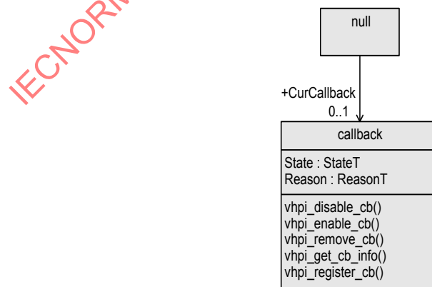
Figure 50—Callbacks class diagram
