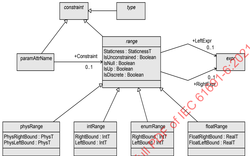
Figure 19—Constraint class diagram
