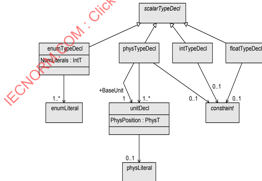
Figure 20—ScalarType class diagram
