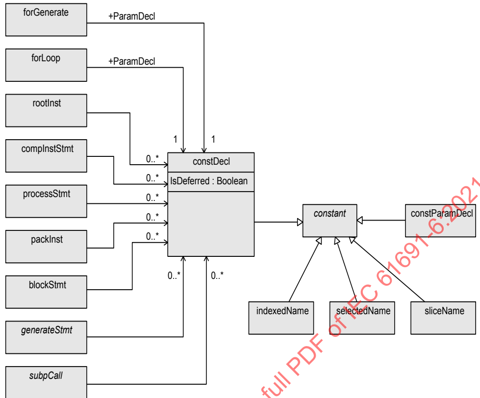
Figure 8—Constants class diagram
