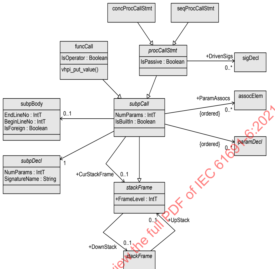
Figure 35—SubCall class diagram
