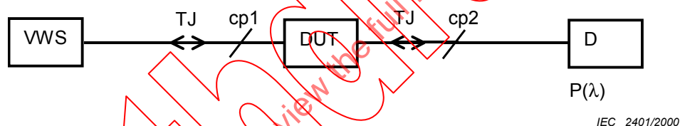
Figure 1 – Optical power meter method – Step 1
