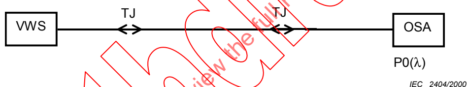
Figure 4 – Optical spectrum analyser method – Step 2
