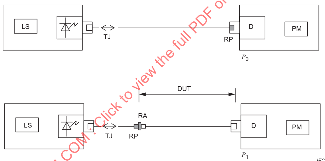
Figure 4 – Insertion method (B) – Type 5 and type 6 DUT
