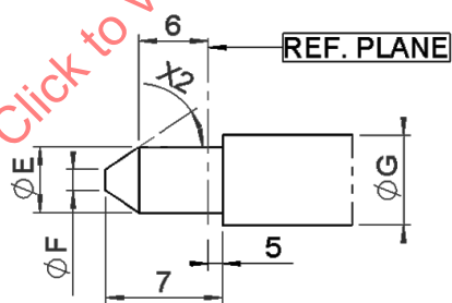
Figure 4 – Details of pin-centre contact (for dimensions, see Table 2)
