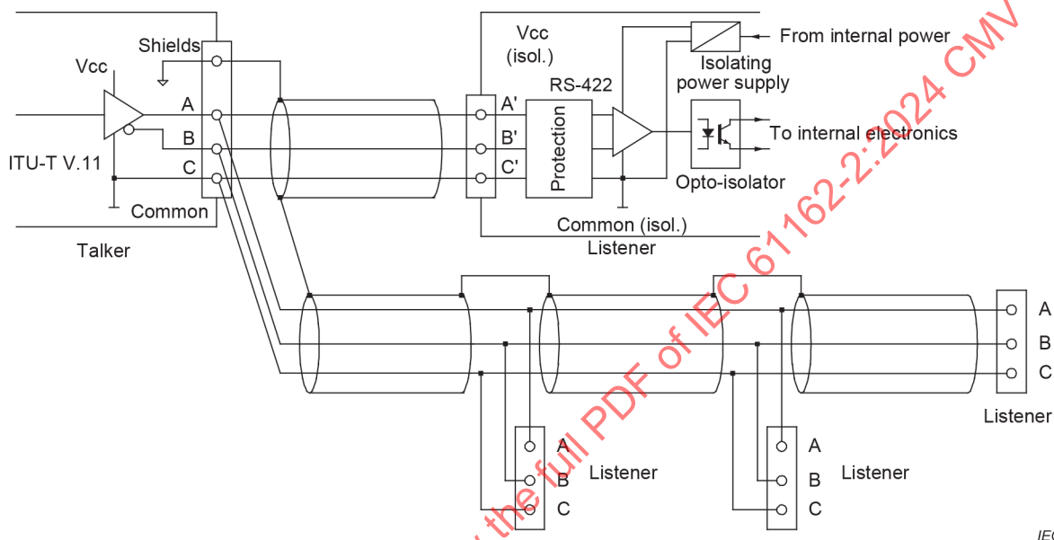
Figure 1 – Talker/listener connections
