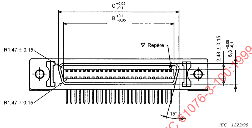
Figure 4 – Embases
