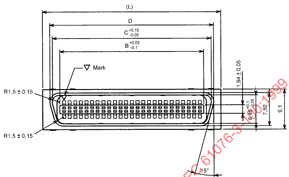
Figure 5 – Free connectors
