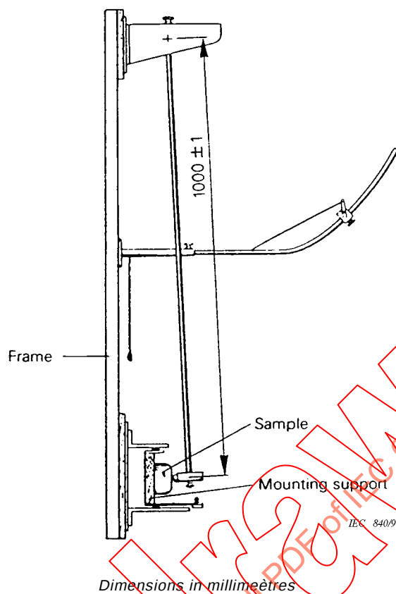
Figure 12 – Mechanical impact test apparatus (9.12.2.1)
