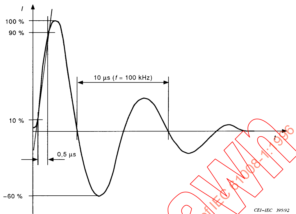
Figure 19a – Current ring wave 0.5 \mu\text{s}/100 \text{ kHz}
