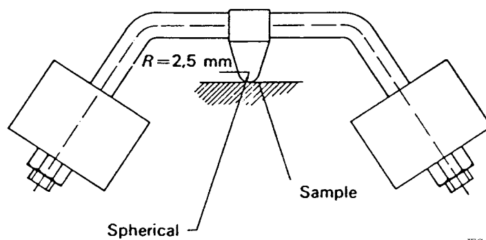
Figure 18 – Ball-pressure test apparatus (9.13.2)
