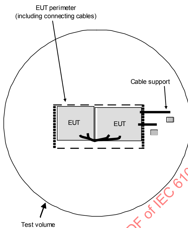
Figure 9 – Example test set-up for floor-standing equipment, top view
