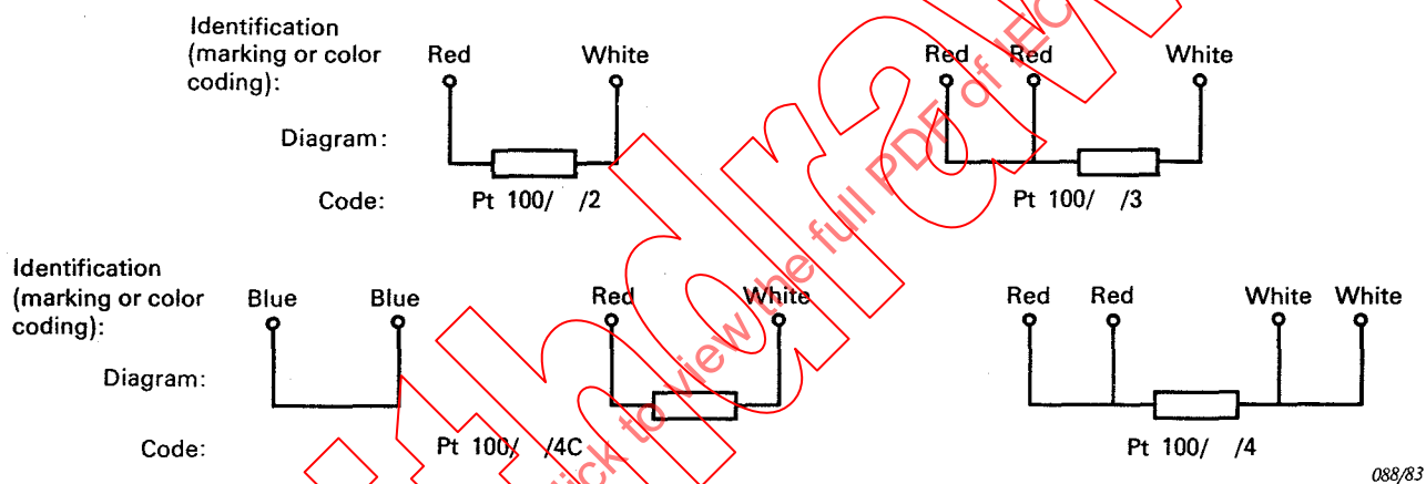
FIG. 3. — Connection configurations.
