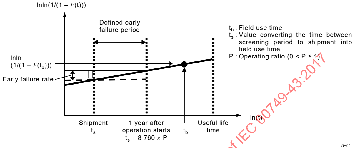
Figure 3 – Weibull conceptual diagram of the early failure rate
