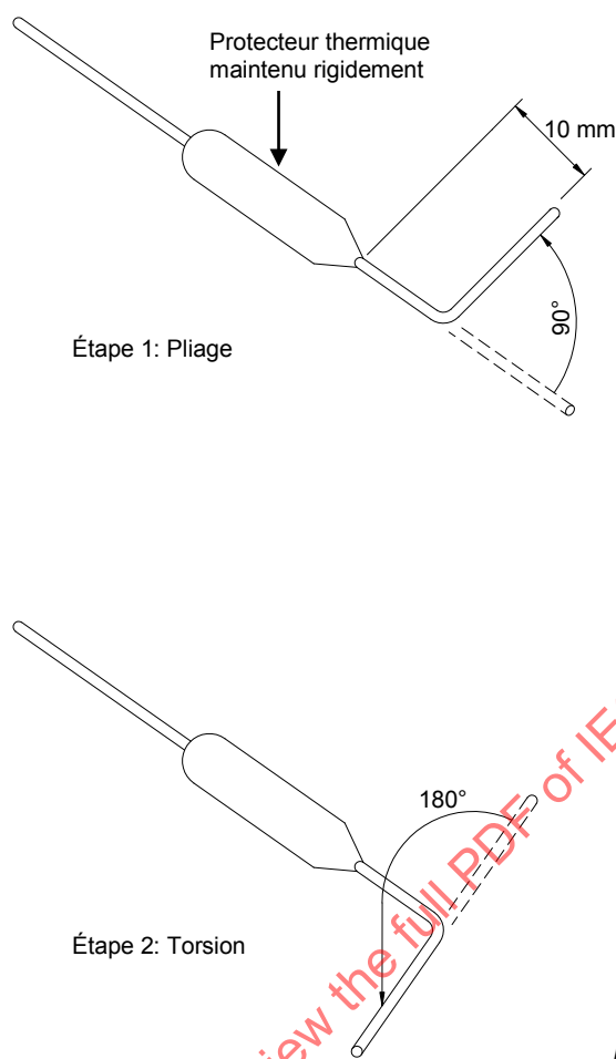
Figure 1 – Essai de torsion
