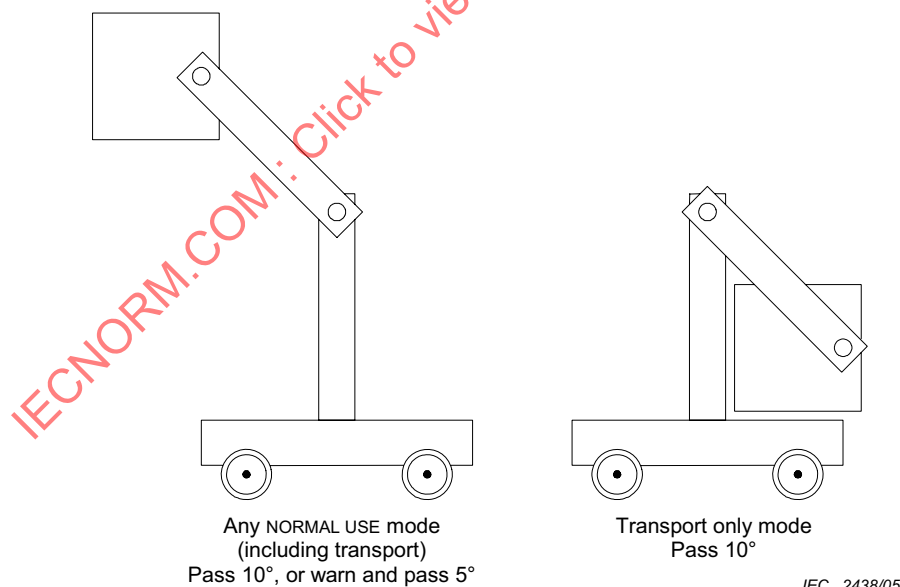
Figure A.16 – Instability test conditions
