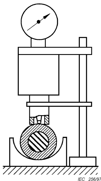
Figure C.2a – Test piece groove
