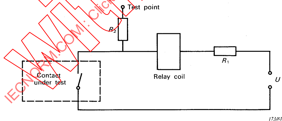
FIG. 2. — D.C. relay load. R_1 : see Sub-clause 4.1. R_2 \geq 50 \text{ k}\Omega
