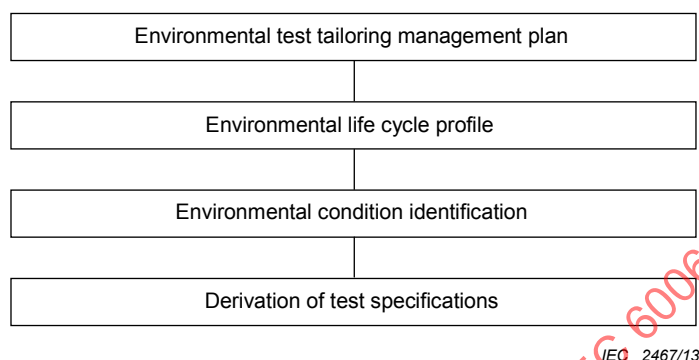
Figure C.1 – Environmental test tailoring process
