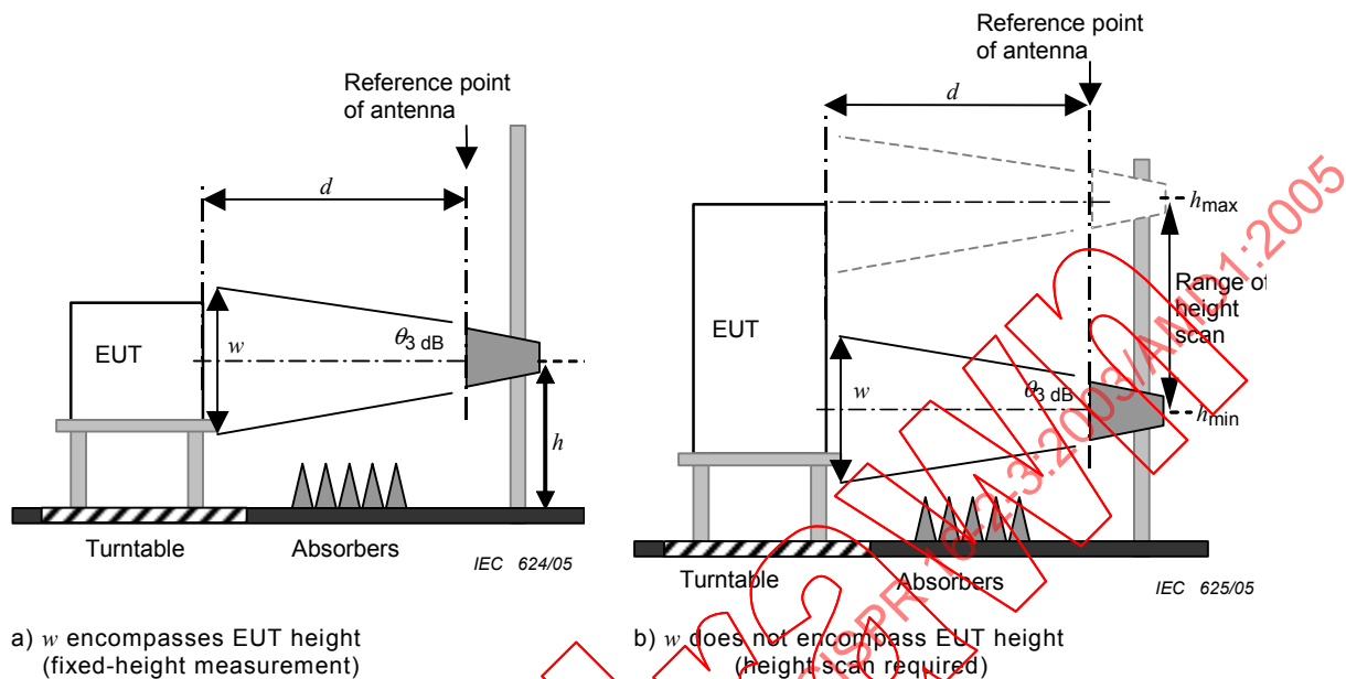
Figure 13 – Illustration of height scan requirements for two different categories of EUTs
