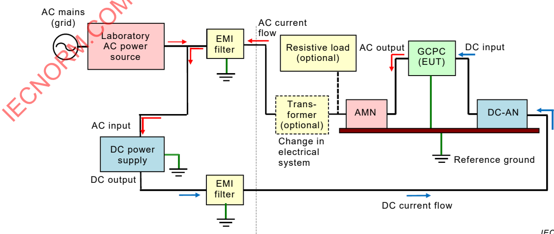
Figure J.1 – Setup of the test site (Case 1) – 2D diagram
