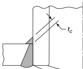
(g) Typical Flush-Type Nozzle
