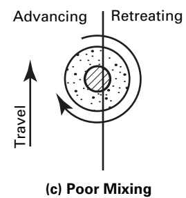
Figure 5 Typical Centered Seam Alignment, Good Mixing by Placing Seam on Advancing Side of Probe, Poor Mixing by Placing Seam on Retreating Side of Probe
