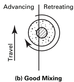
Figure 5 Typical Centered Seam Alignment, Good Mixing by Placing Seam on Advancing Side of Probe, Poor Mixing by Placing Seam on Retreating Side of Probe
