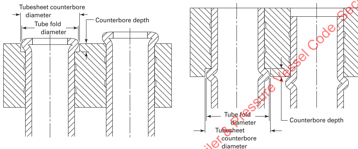
Figure 1 Typical Tube-to-Tubesheet Configurations Prior to Welding
