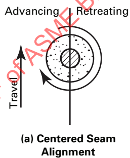
Figure 5 Typical Centered Seam Alignment, Good Mixing by Placing Seam on Advancing Side of Probe, Poor Mixing by Placing Seam on Retreating Side of Probe
