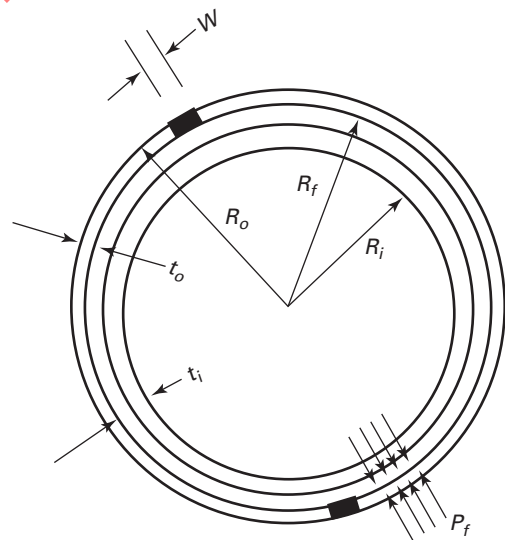
Figure 9 Layered Vessel
