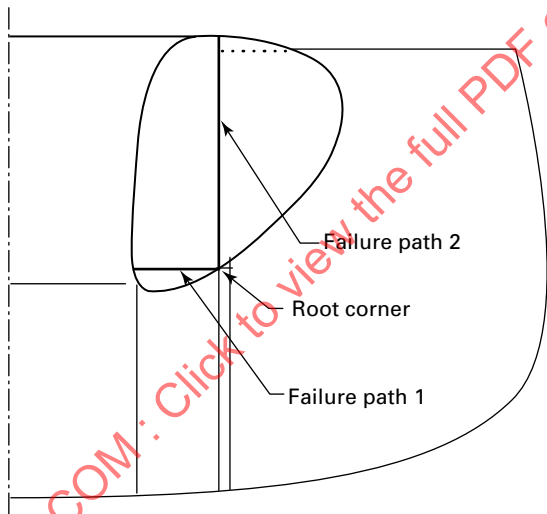
Figure 2 Weld Leg
