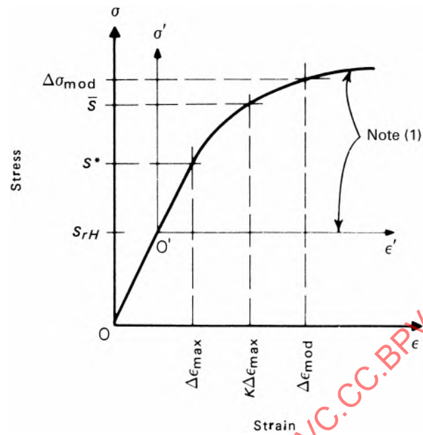
Figure 10 Stress-Strain Relationship
