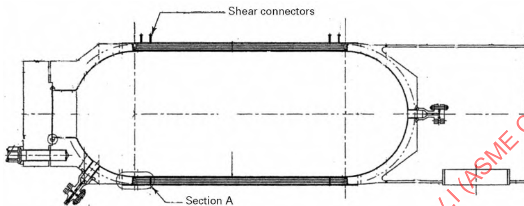
Figure 1 Example of Steel-Layered Vessel
