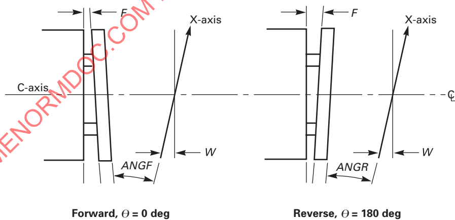
Fig. 7.8.2.1-2 Schematic Showing the Angles Involved When Measuring Cross-Slide Squareness to the Spindle Axis
