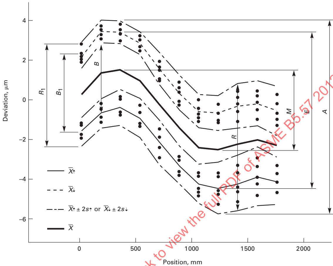
Fig. 7.2.7-1 The Full Data Set for the Positioning Deviations of an Axis
