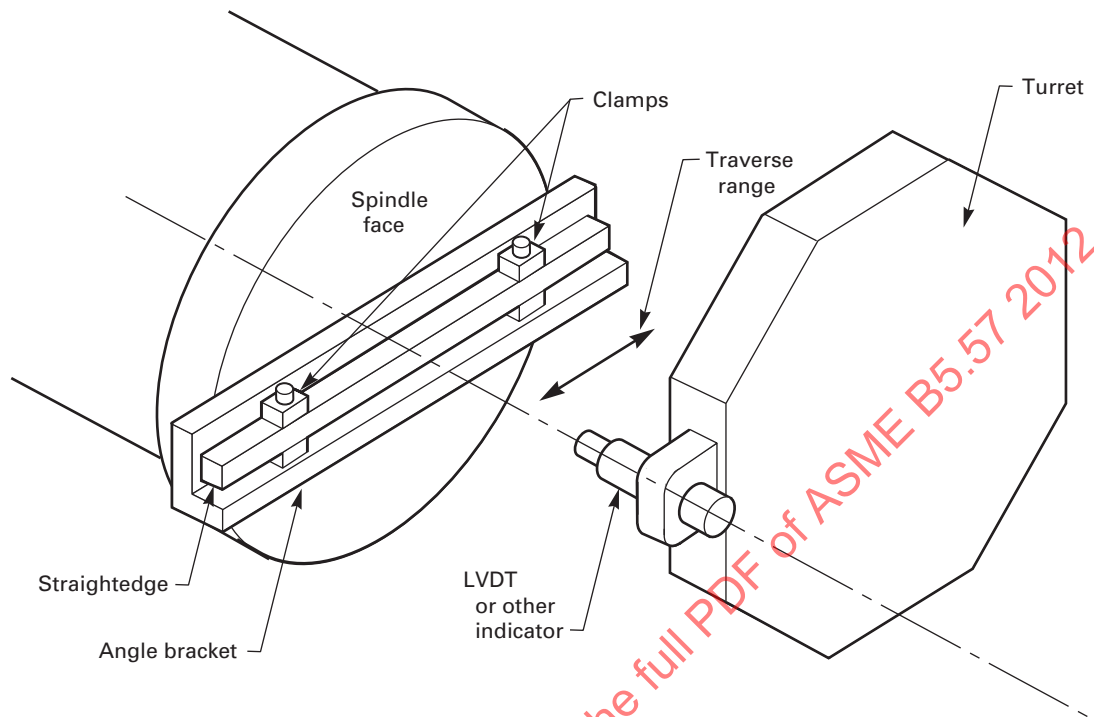
Fig. 7.8.2.1-1 Setup for Measuring Squareness of the Cross-Slide to the Work Spindle Using a Mechanical Straightedge
