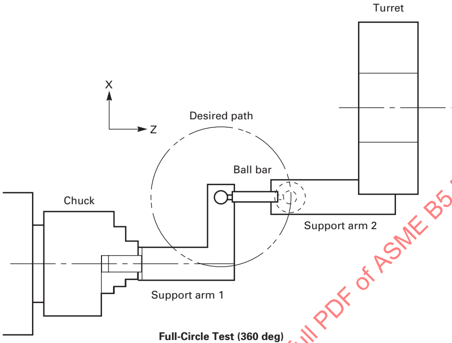
Fig. 7.9.2-1 Typical Setup for a 360-deg Ball Bar Test
