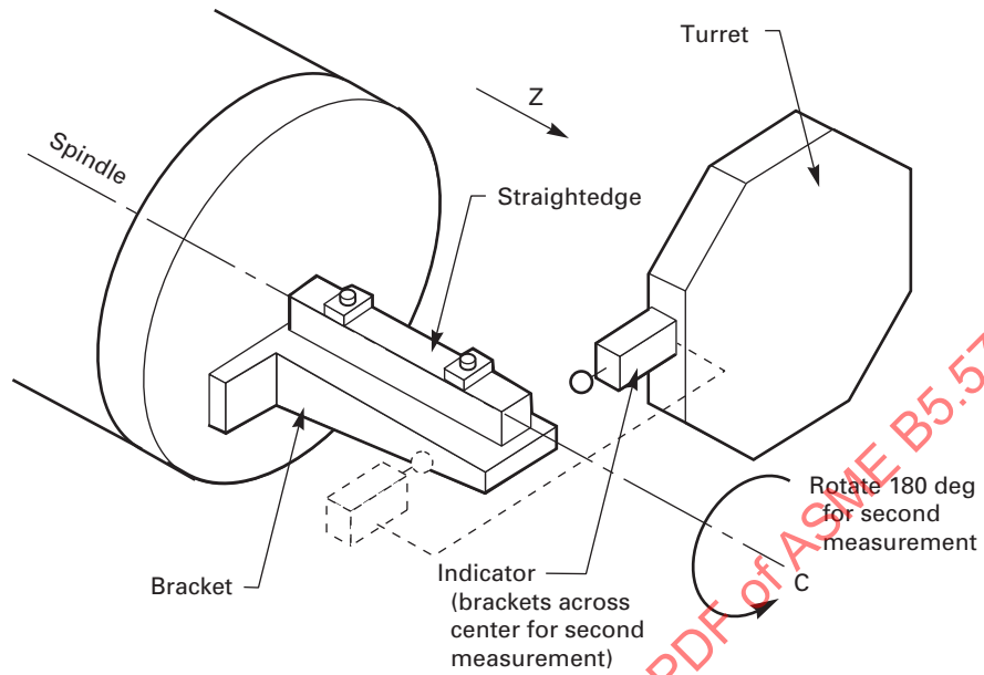
Fig. 7.8.3.1-2 Setup for Straightedge Rotation on a Horizontal Spindle Lathe for Measuring Z-Axis Parallelism to the C-Axis
