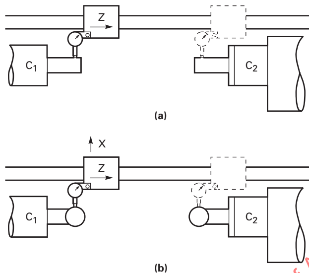
Fig. 8.2.5.1-1 Setup for Measuring Tail Stock Alignment Using the In-Feed (Z) Axis
