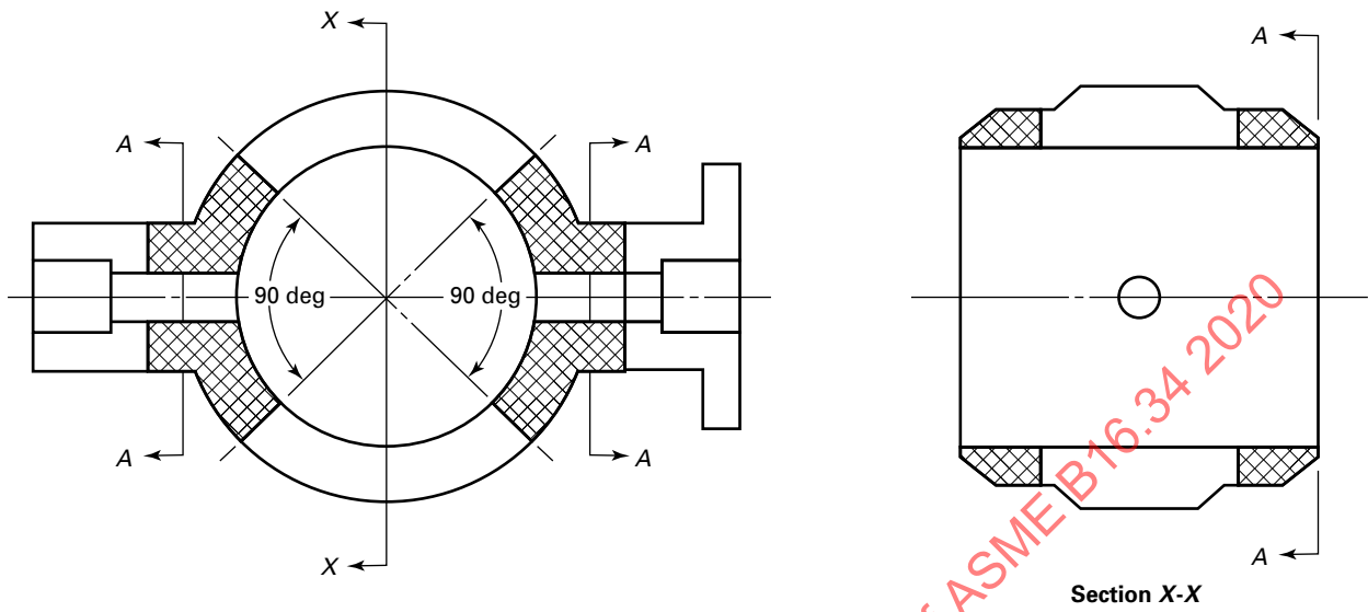
Figure 13 Butterfly Body
