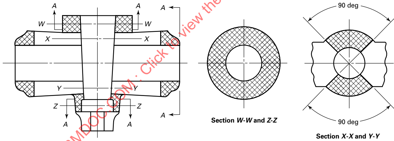
Figure 14 Plug Body
