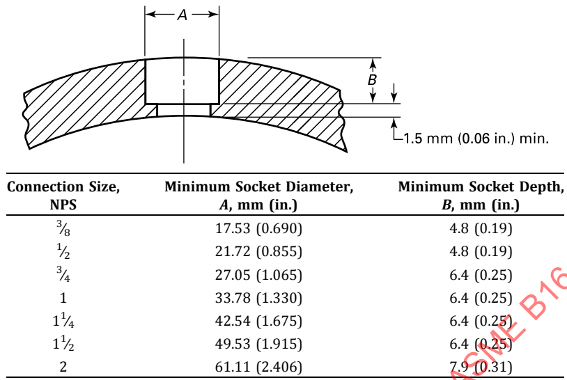
Figure 5 Socket Welding for Auxiliary Connections
