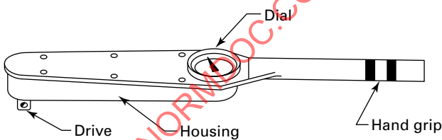
Figure 5.1.1-3 Category 14, Type I, Class C
