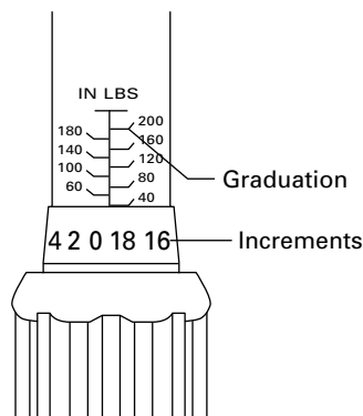
Figure 6.1-1 Graduated Range
