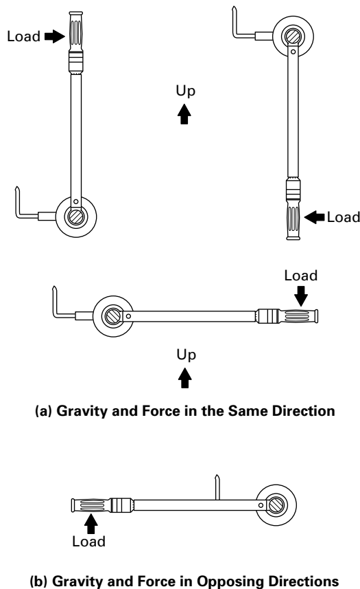
Figure 6.6.2-1 Gravity-Dependent Test Positions
