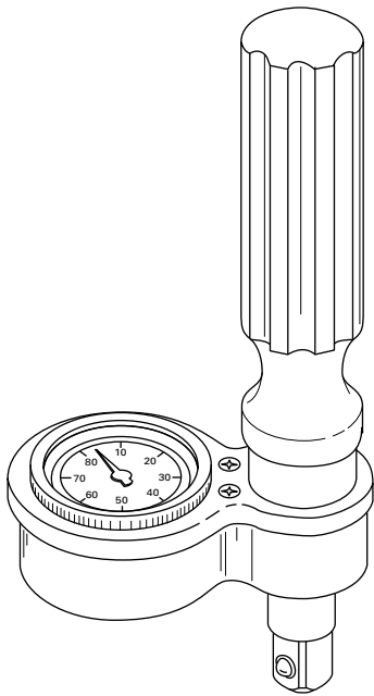
Figure 5.1.2-1 Category 14, Type I, Class E, Style 1
