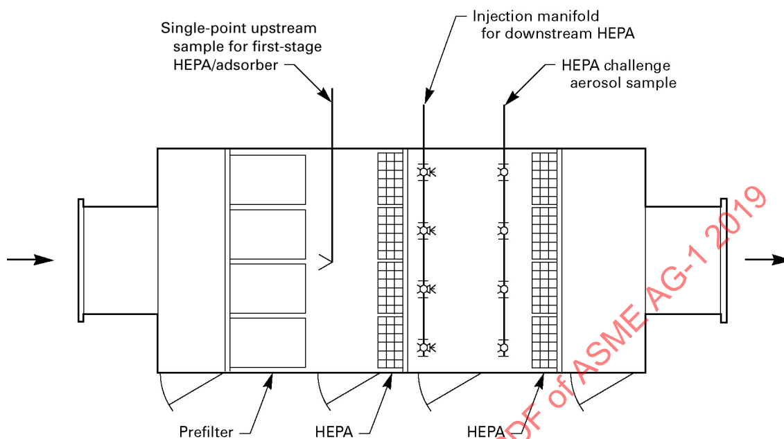
Plan C: Ducted Inlet/Outlet HEPA/HEPA Configuration
