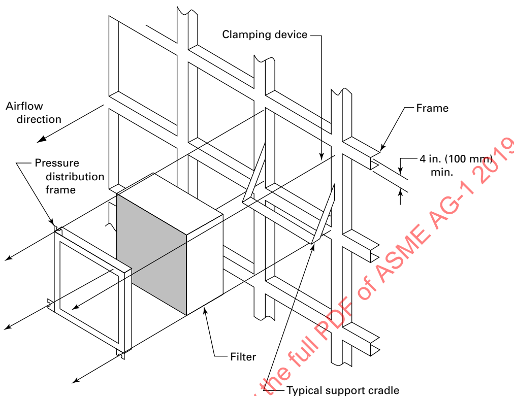
Figure FG-4110-1 Typical Filter Mounting Frame
