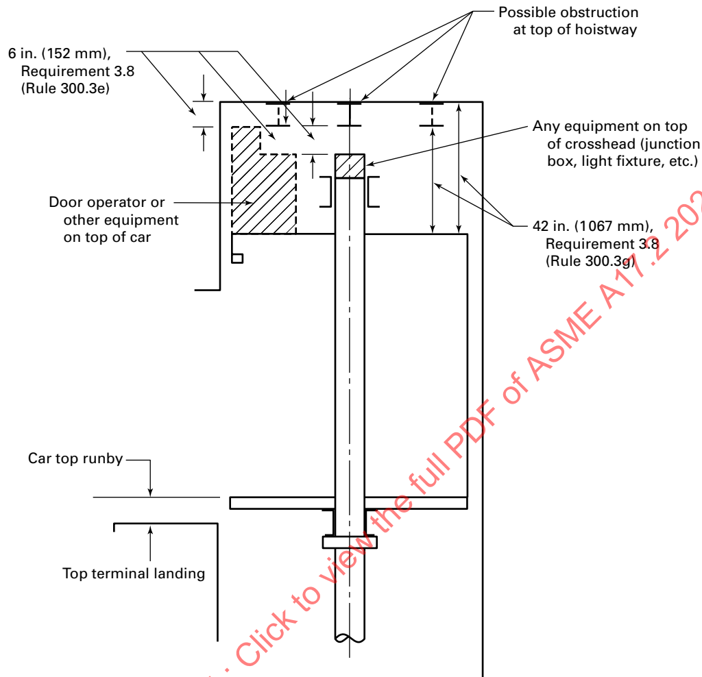
Figure 3.4.1.2 Car Top Clearance and Runby (A17.1-1978 and Later Editions)
