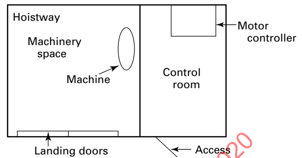
Figure 11.21(a) Configuration A
