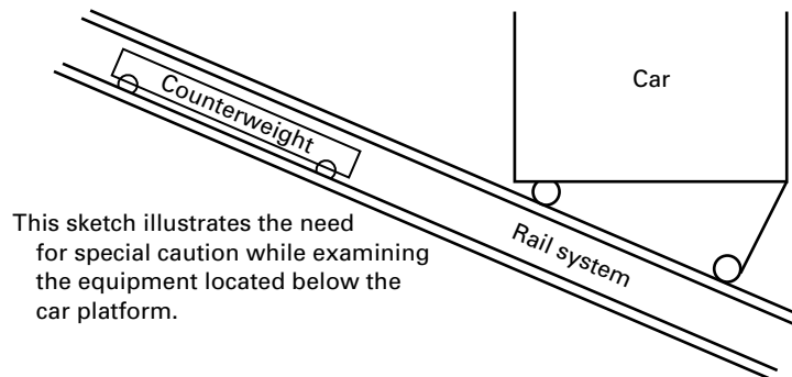
Figure I-3.4 Uphill Clearance
