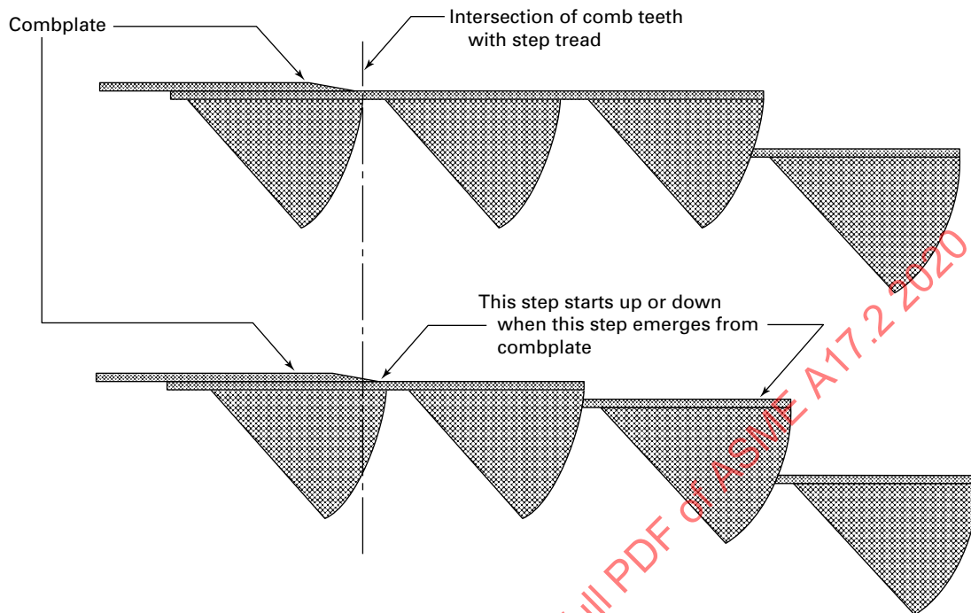
Figure 7.9.3 Example of Two Flat Steps
