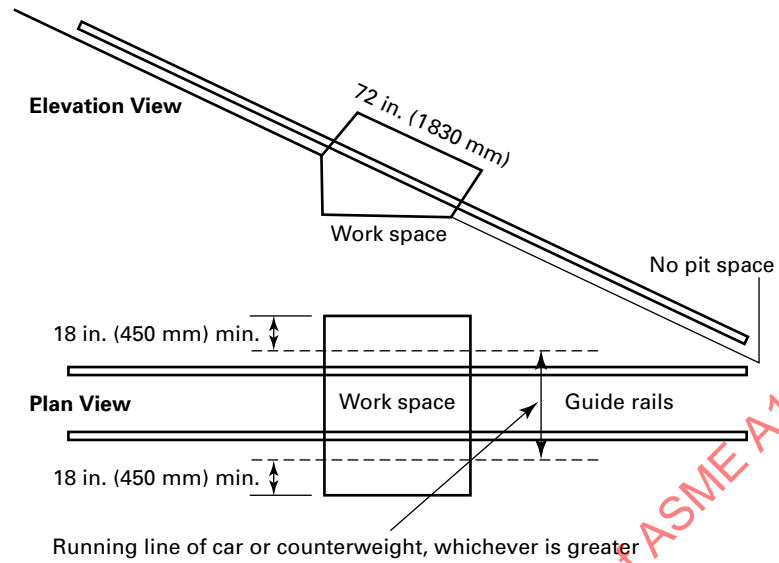
Figure I-5.1.1.3 Pits and Work Spaces
