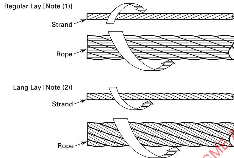
Figure 3.23.1(a) Types of Lay
