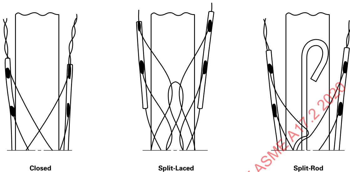
Figure 3.16.1 Self-Tightening Grips
