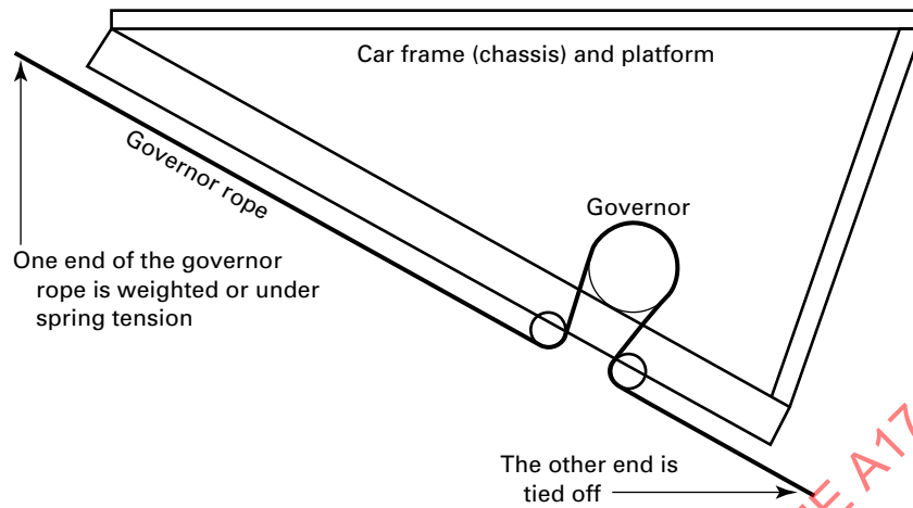
Figure I-2.13.2.3(a) Static Governor-Rope Drive
