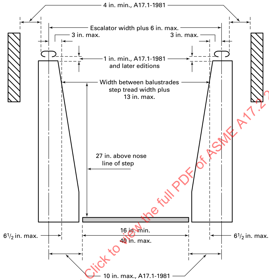
Figure 7.2.1(b) Dimensions for Existing Escalators (for Escalators Installed Under A17.1-1965 Through A17.1-1981)
