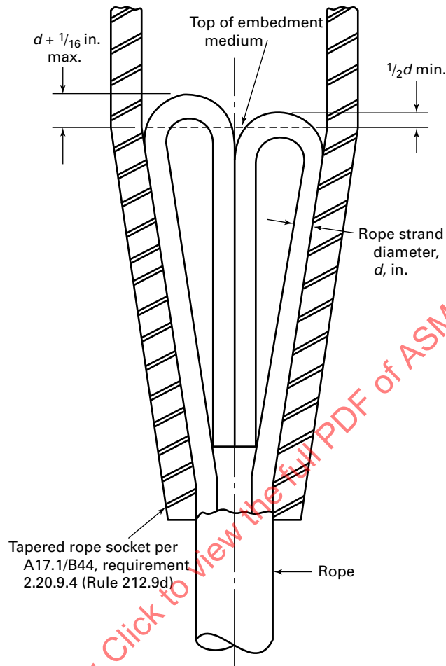
Figure 3.22.1 Cross Section Through Tapered Rope Socket Showing Maximum and Minimum Projection of Loops Above Embedment Medium
