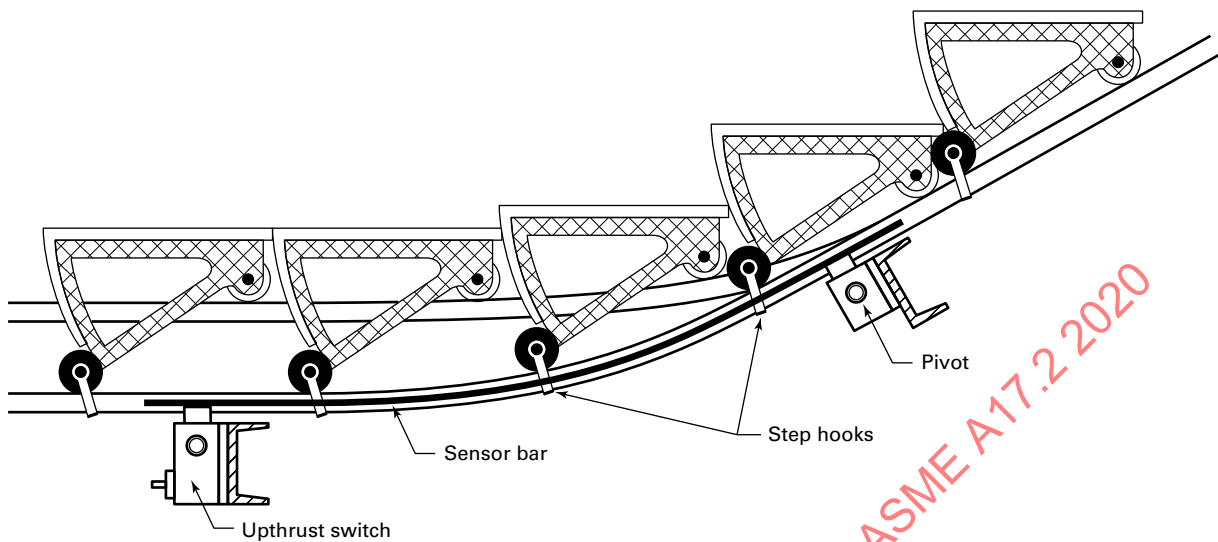
Figure 8.9.2 Typical Step Upthrust Device
