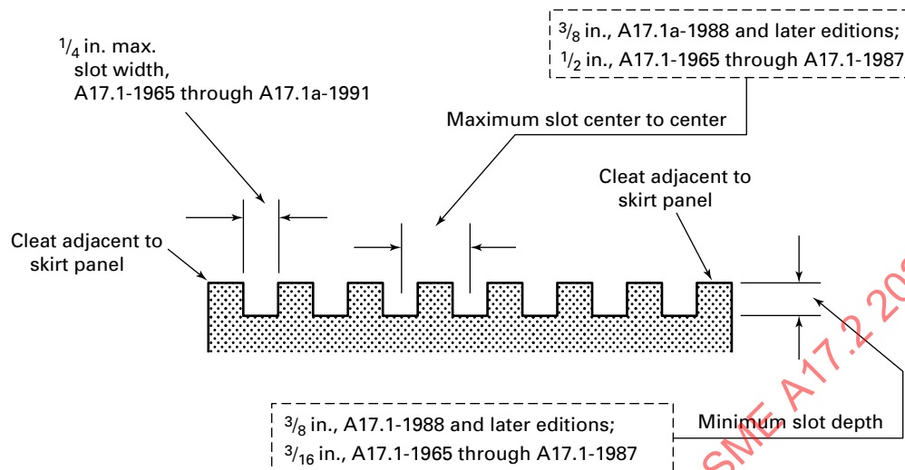
Figure 9.9.1 Moving Walk Treadway Slots
