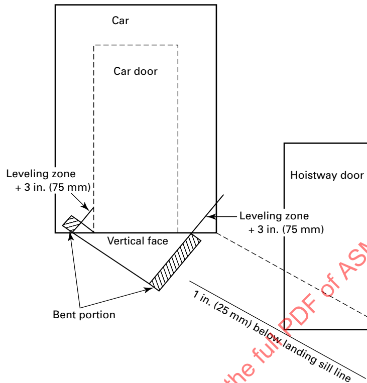
Figure I-4.1 Car Platform Guard
