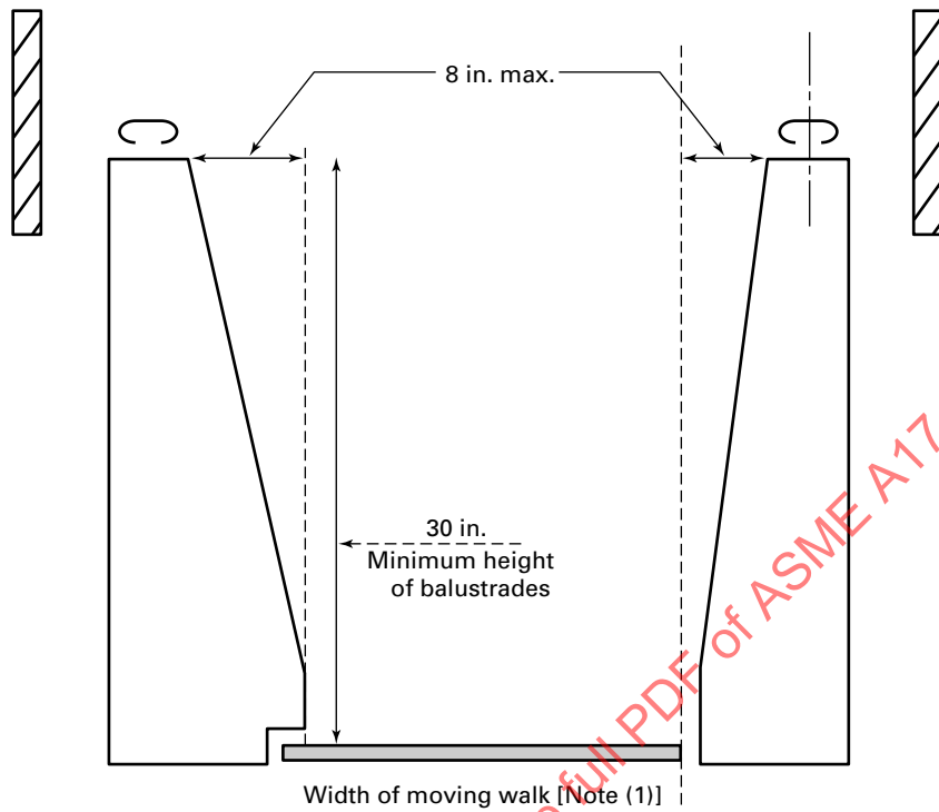
Figure 9.2.1(a) Moving Walk Geometry (for Moving Walks Installed Under A17.1-1965 Through A17.1b-1980)
