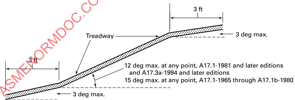
Figure 9.2.3 Maximum Treadway Angle
