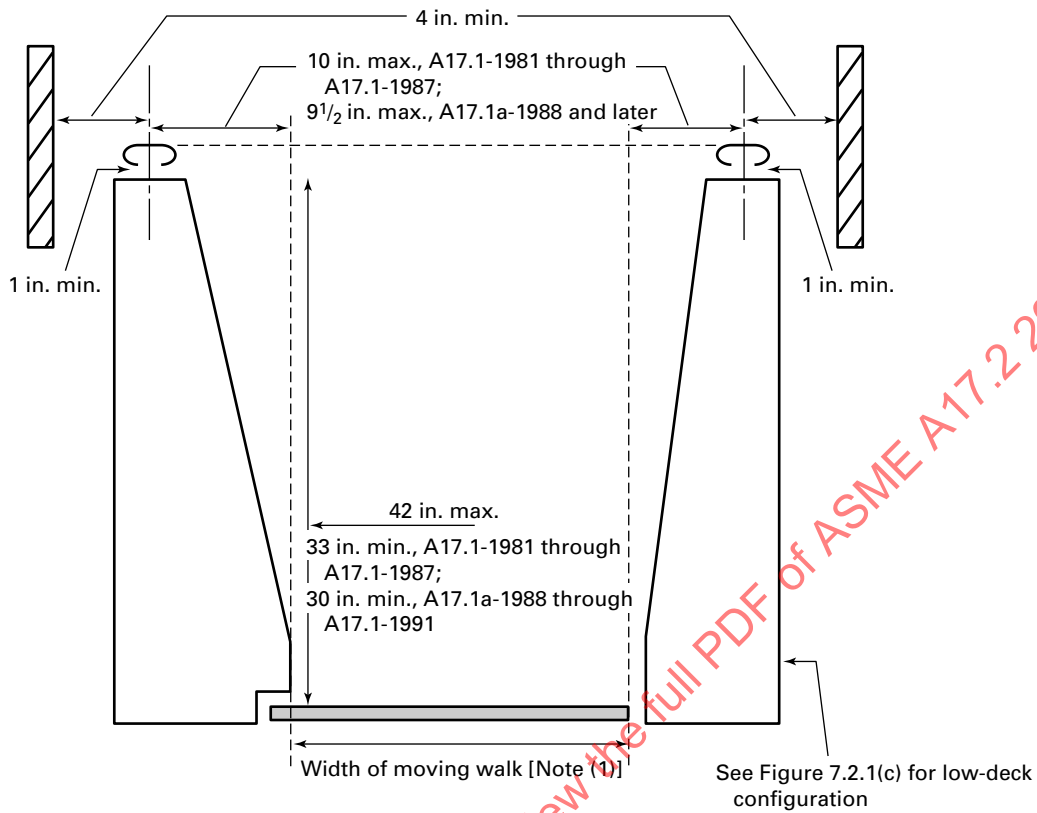
Figure 9.2.1(b) Moving Walk Geometry (for Moving Walks Installed Under A17.1-1981 Through A17.1a-1991)
