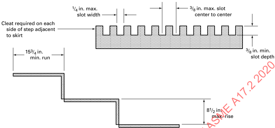
Figure 7.9.1(d) Escalator Step Tread [A17.1-1955 Through A17.1-1990, Rule 802.5 (Requirement 6.1.3.5)]
