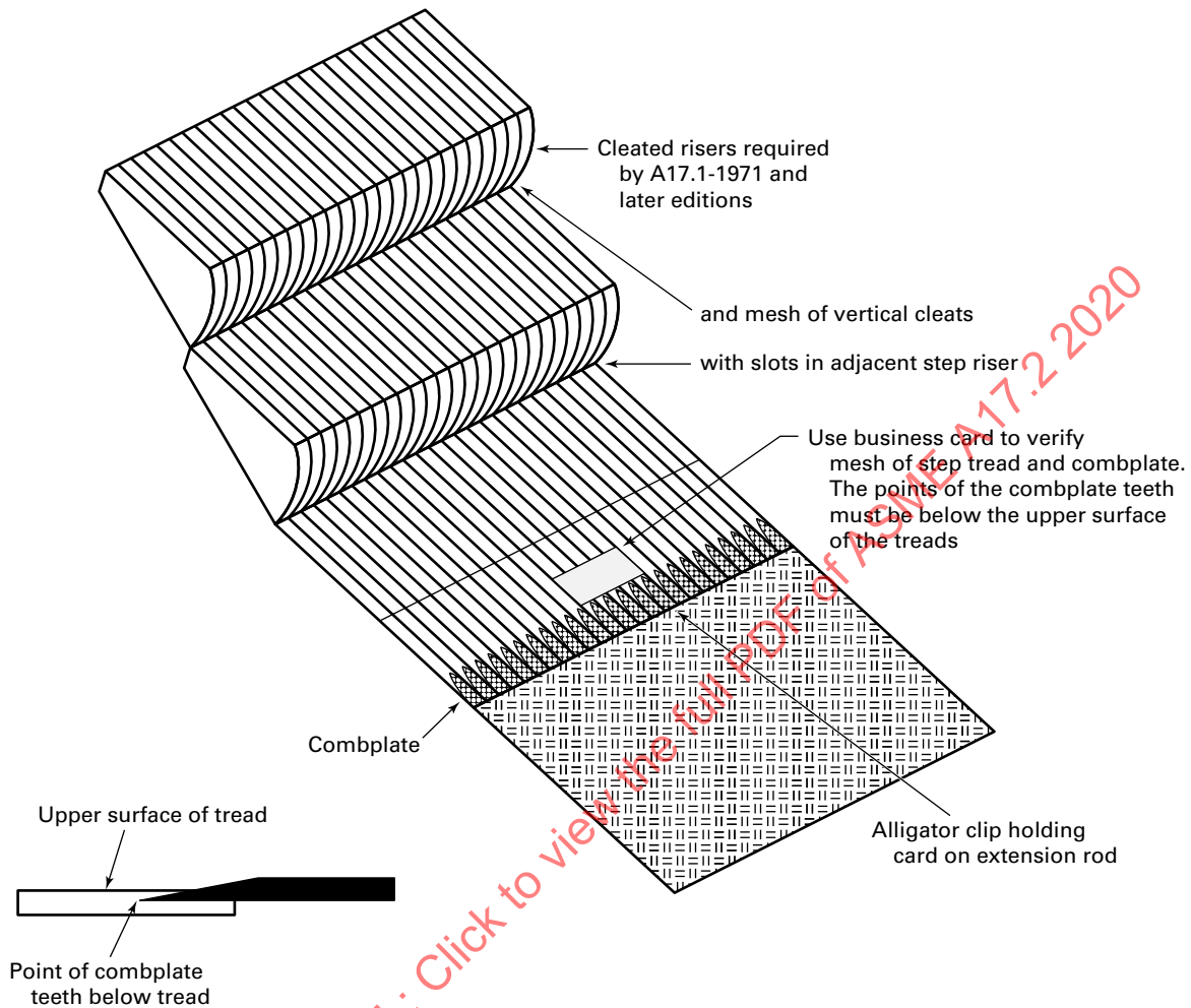
Figure 7.7.1 Checking Step/Combplate Mesh
