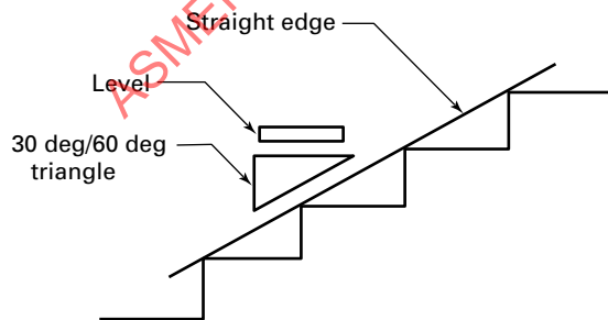
Figure 7.2.3 Checking Incline
