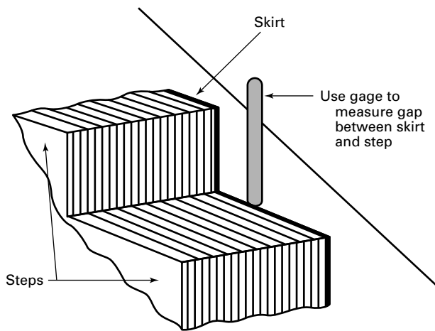
Figure 7.17.1 Measuring Gap Between Step and Skirt
