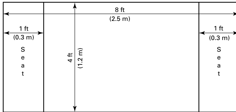
Figure I-1.16.3.3 Net Platform Area Measurements
