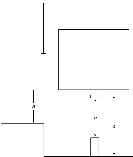
Figure 5.2.3.1 Bottom Car Clearance Electric and Hydraulic Elevators
