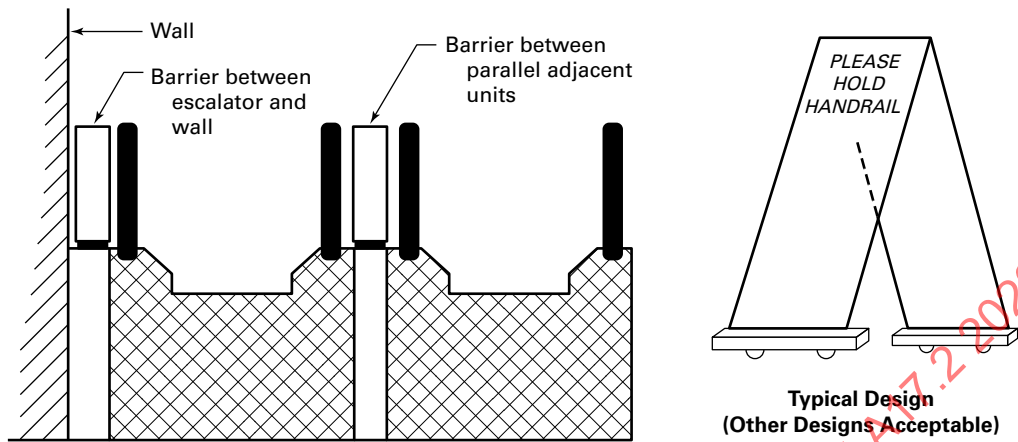
Figure 7.8.1(a) Deck Barricade
