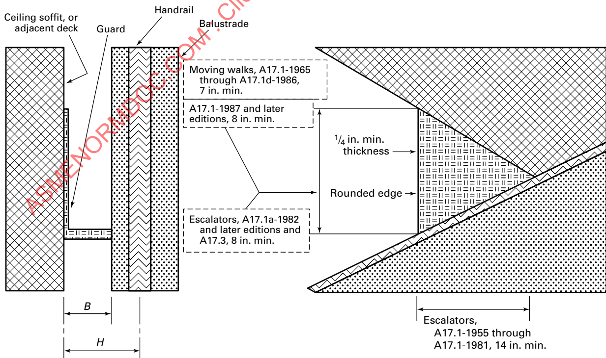
Figure 7.16.1 Ceiling or Soffit Guard [Requirements 6.1.3.3.9 and 6.2.3.3.7 (Rules 802.3g and 902.3g)]
