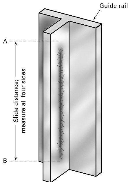
Figure 2.29.2(b) Safety Marks on Guide Rails, Good Illumination
