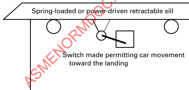
Figure I-2.28.2.3 Retractable Sill
