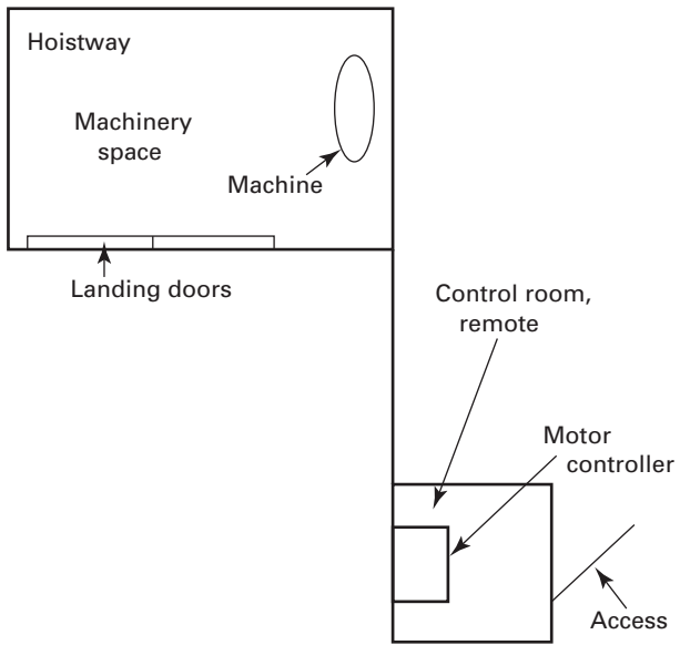
Figure 11.21(d) Configuration D
