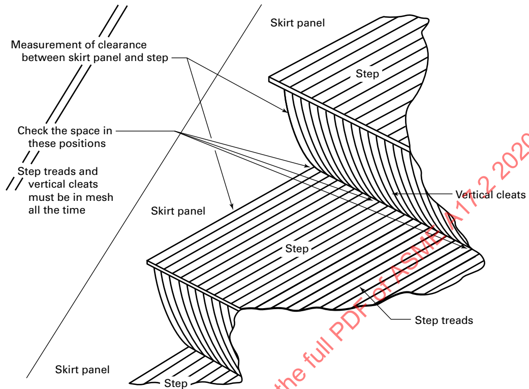
Figure 7.9.1(b) Cleated Riser
