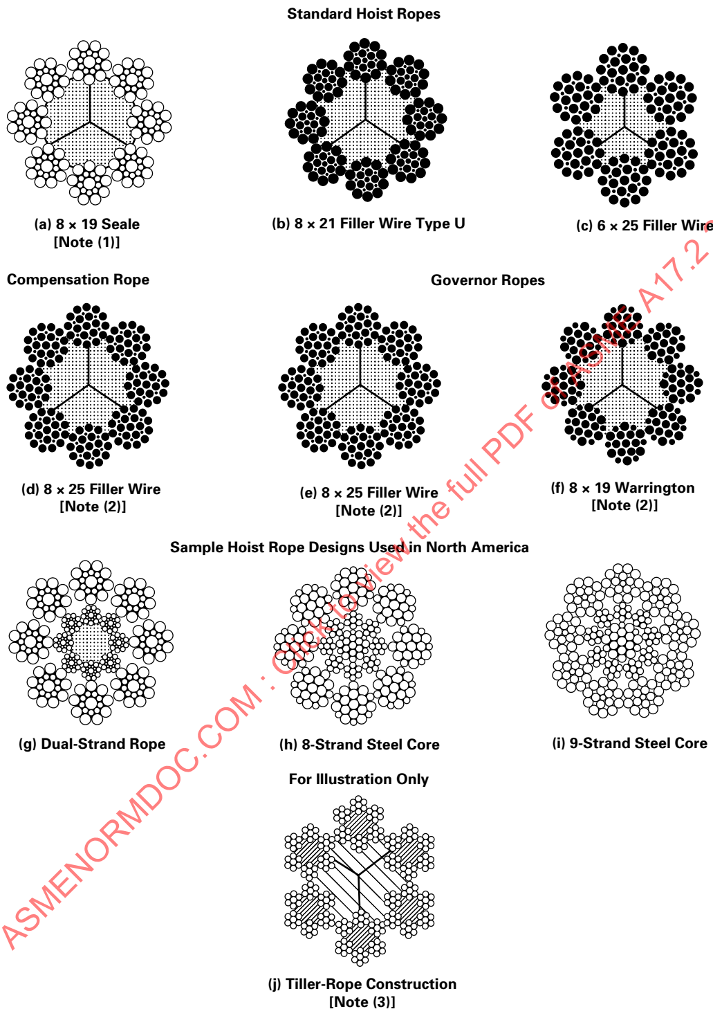
Figure 3.23.1(b) Cross Sections of Typical Wire Ropes
