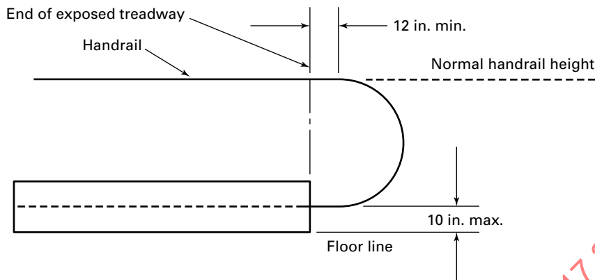
Figure 9.3.3 Moving Walk Handrail Extension (A17.1-1971 and Later Editions)
