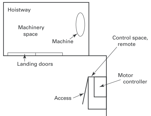
Figure 11.21(c) Configuration C
