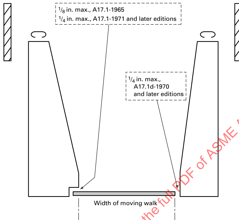
Figure 9.15.1 Treadway Clearances
